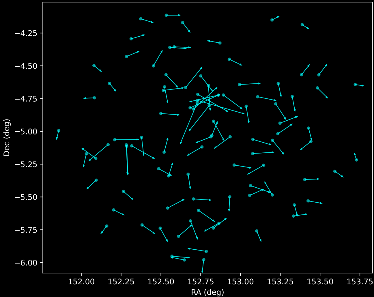
GALAH DR4 Noise Stream Proper Motion Vectors (n=95)
