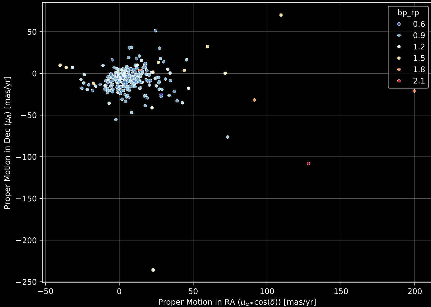
GALAH DR4 Field: [7063] Proper Motion Diagram (n= 296)
