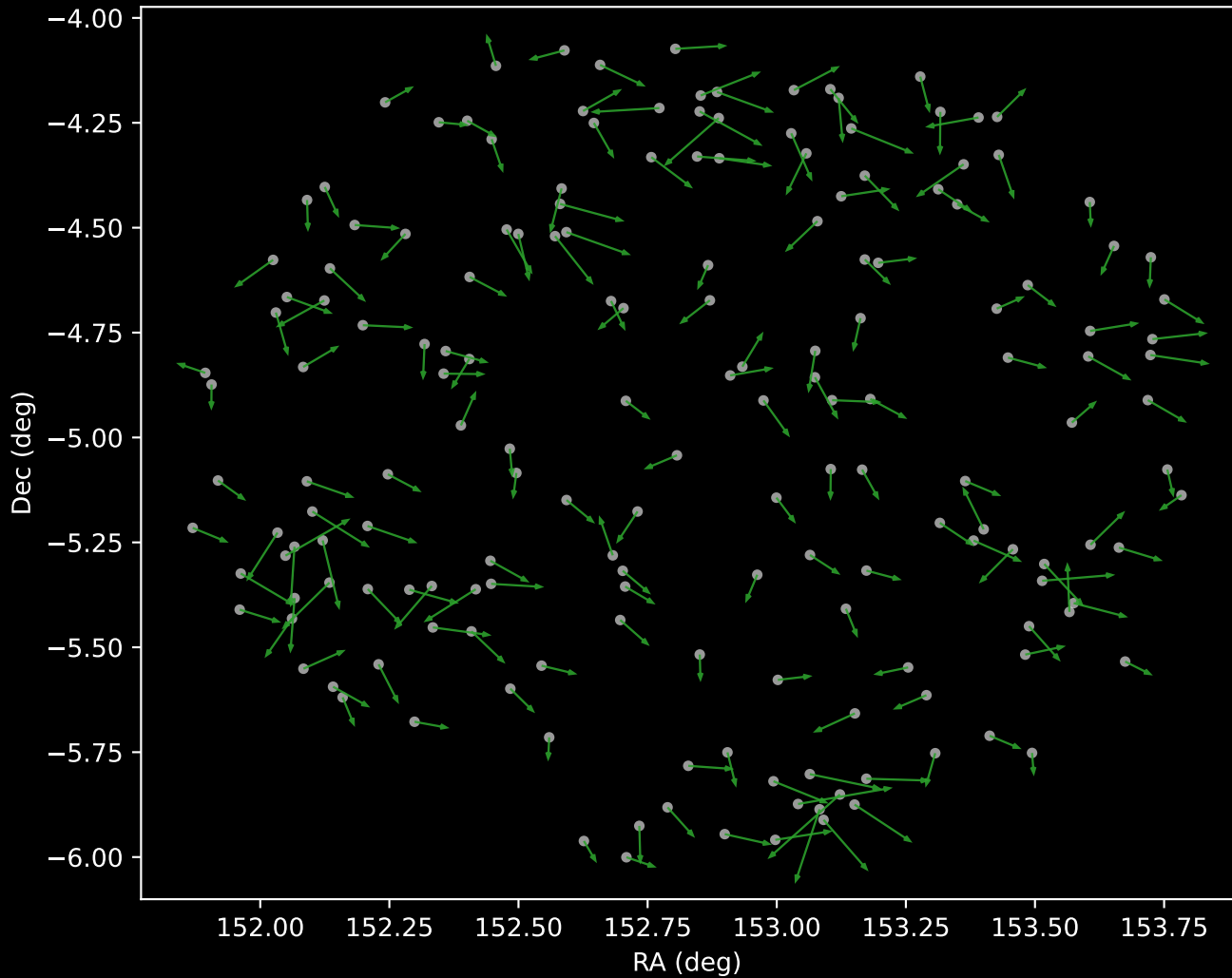
GALAH DR4 Cluster 4 Proper Motion Vectors (n=175)
