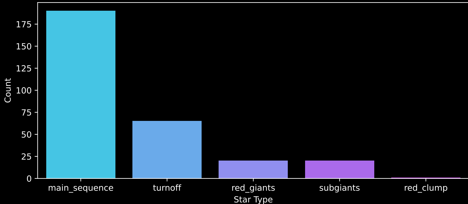
GALAH DR4 Field: [7063] Count plot of Star Type
