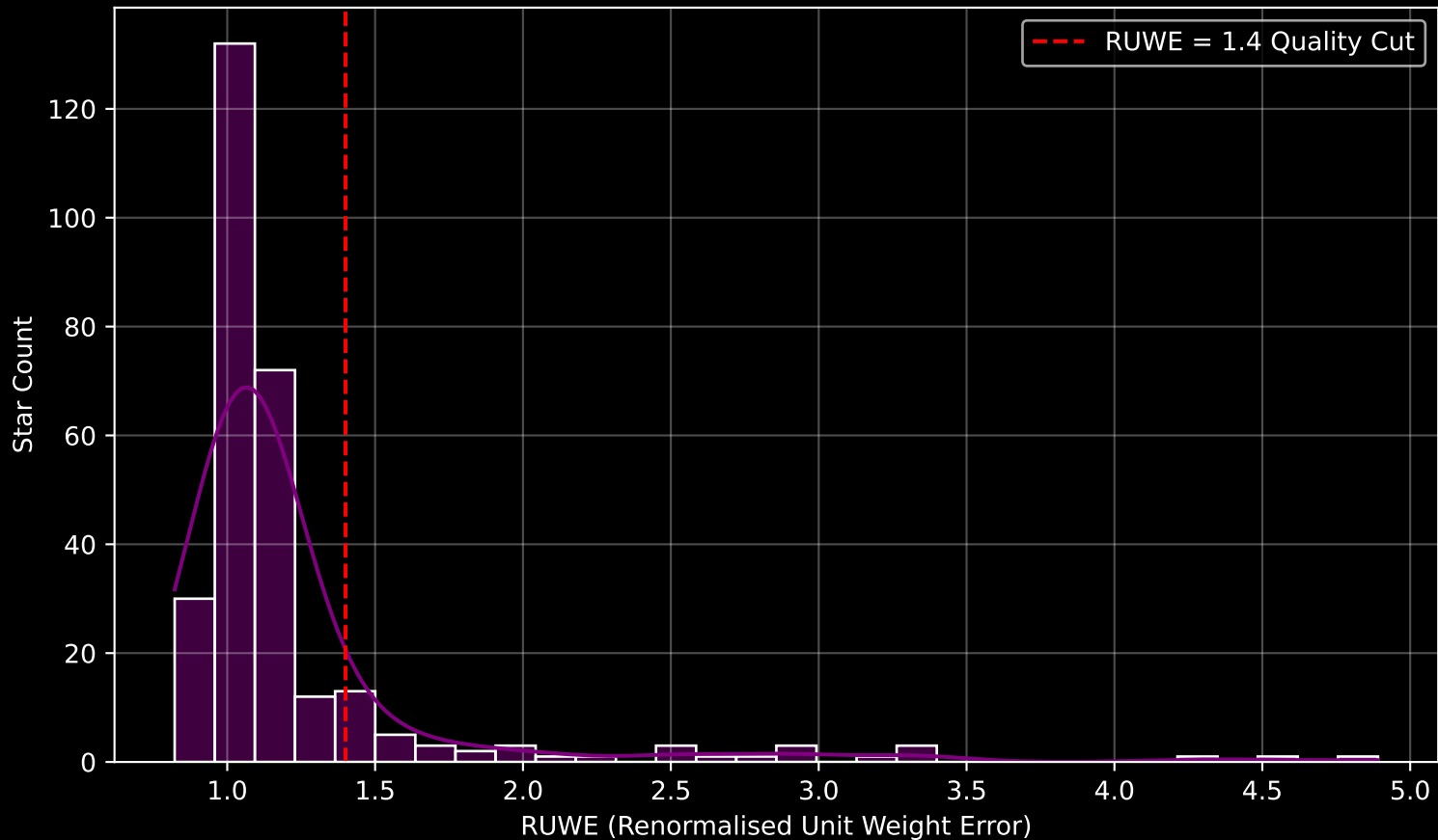
GALAH DR4 Field [7063] RUWE Distribution (n= 289)
