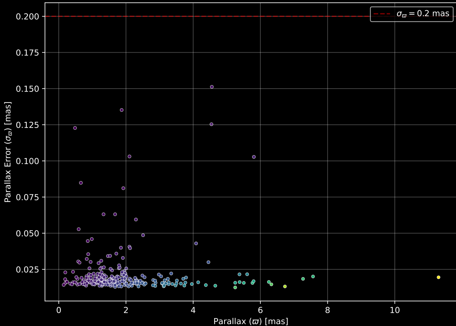
GALAH DR4 Field: [7063] Parallax Quality (n= 296)
